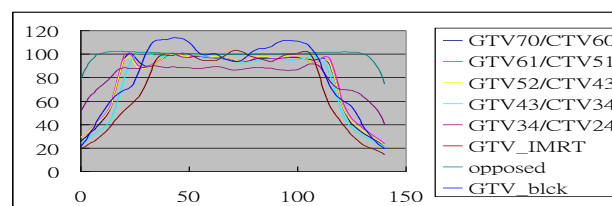
Fig1 Beam uniformity across target
